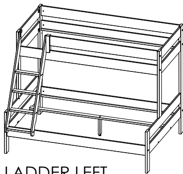
LADDER LEFT
